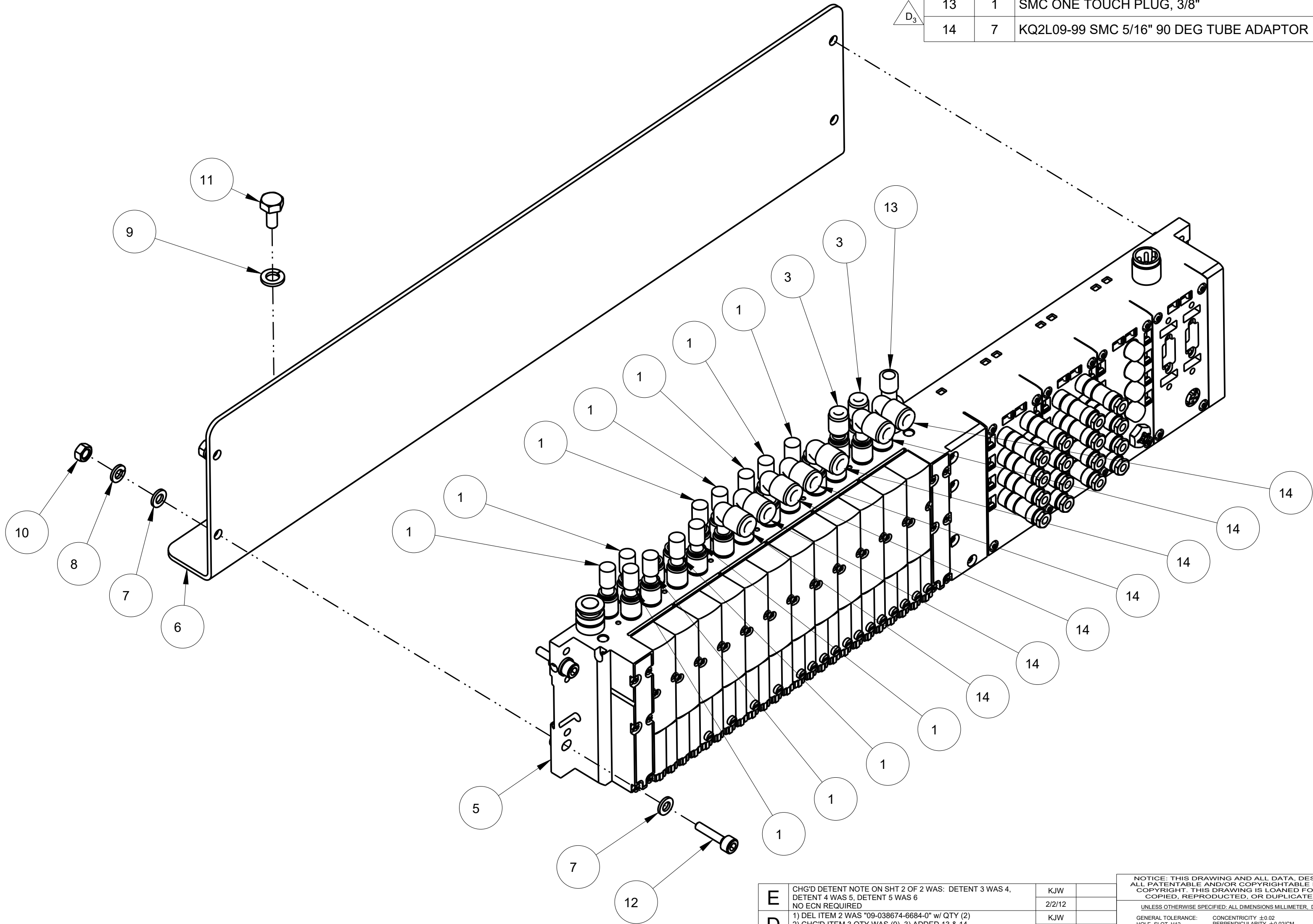
ISO VIEW SCALE 1/2
